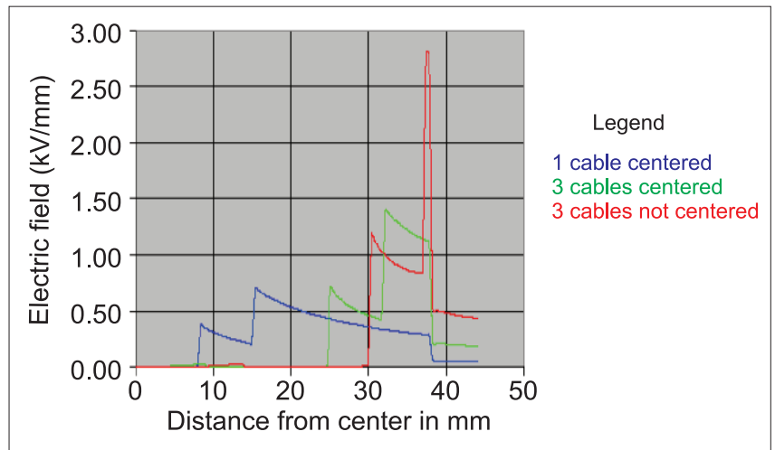
Electric Field Shielding Effects
