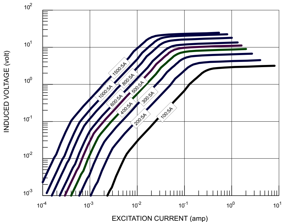
TYPICAL EXCITATION CURVE for MODEL 2562 at 60HZ
