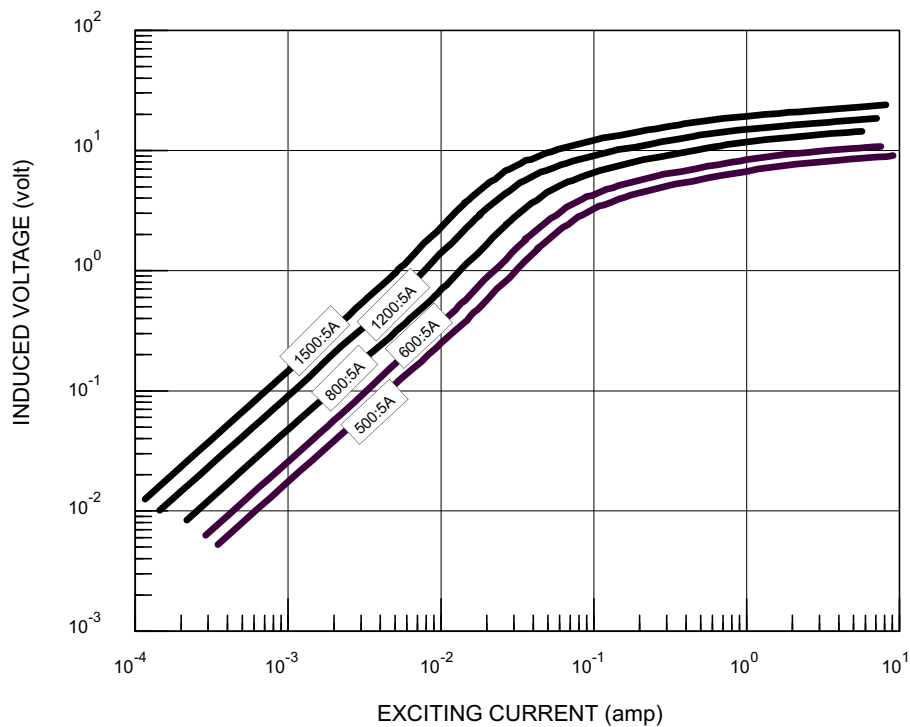
TYPICAL EXCITATION CURVE for MODEL 2743 at 60HZ
